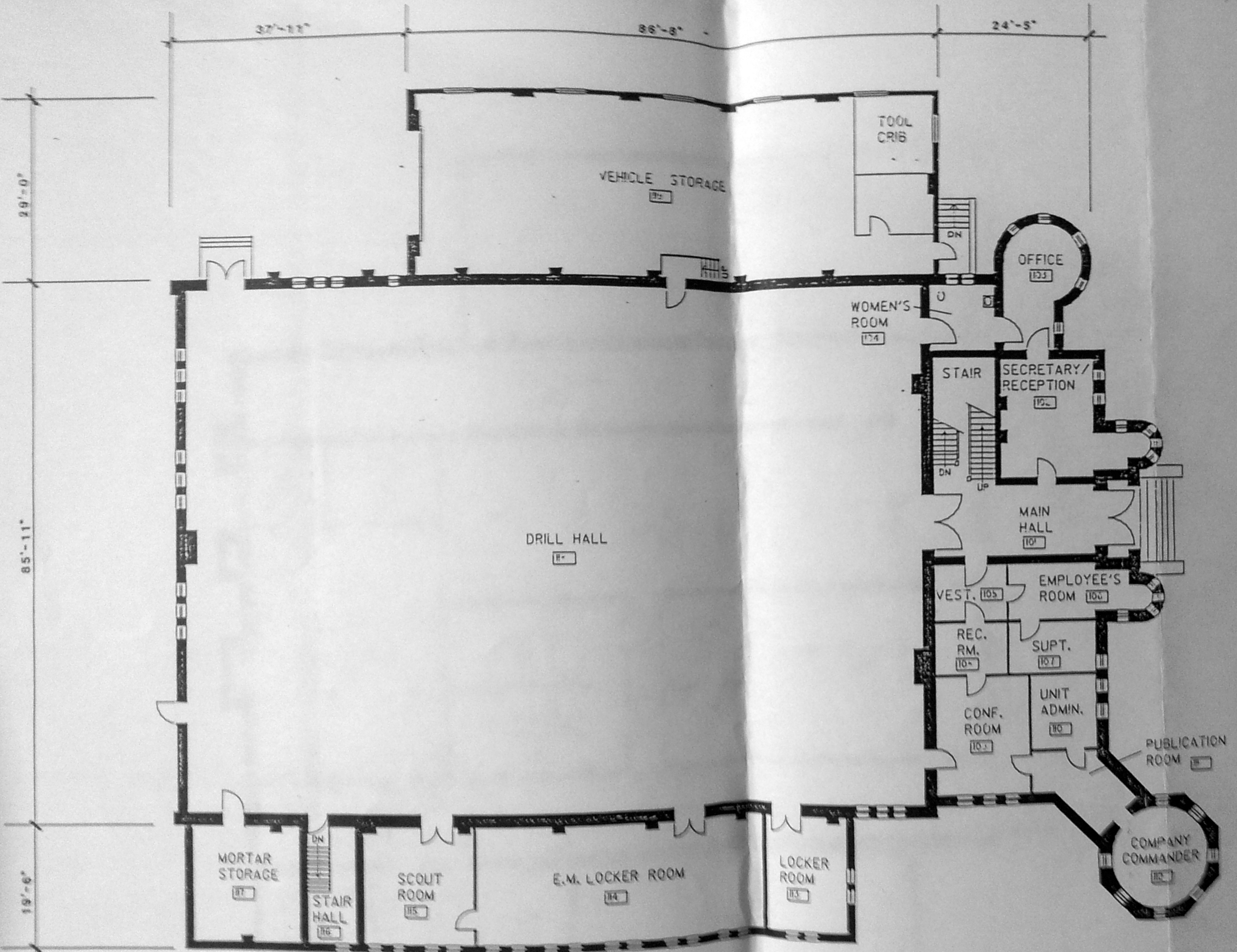
STATE ARMORY AMSTERDAM, N.Y. FIRST FLOOR PLAN SCALE: 1/16" = 1'-0" DATE: AUGUST, 1989
